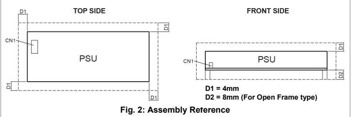
Fig. 2: Assembly Reference
