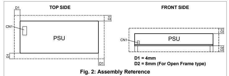
Fig. 2: Assembly Reference
