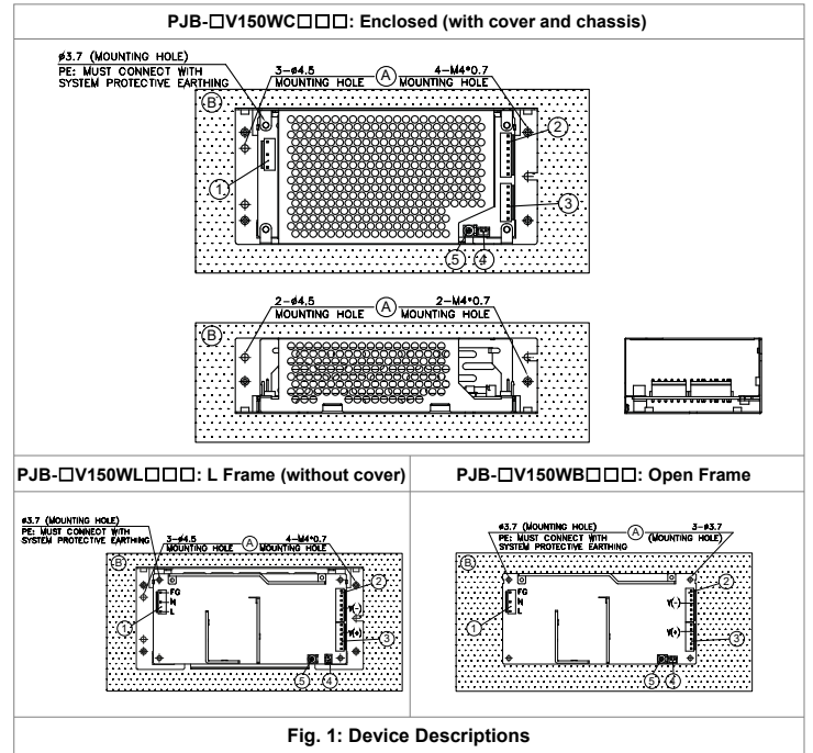
Fig. 1: Device Descriptions
