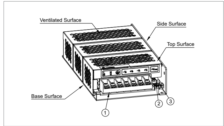
Fig. 1. Device Descriptions
